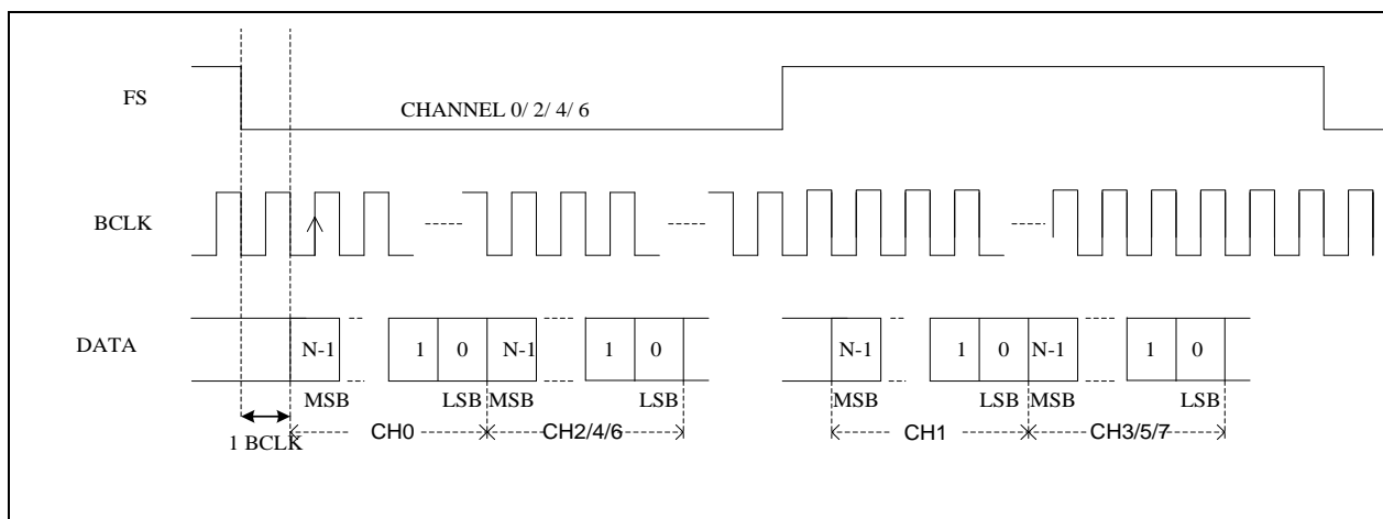
Figure 24 TDM I2S Audio Data
